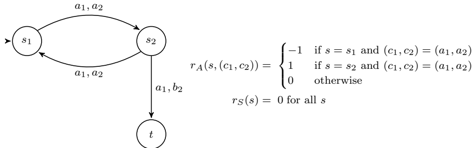
Fig. 13: Counterexample for zero-sum expected reachability reward properties.
