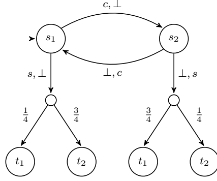
Fig. 14: Counterexample for nonzero-sum probabilistic reachability properties.
