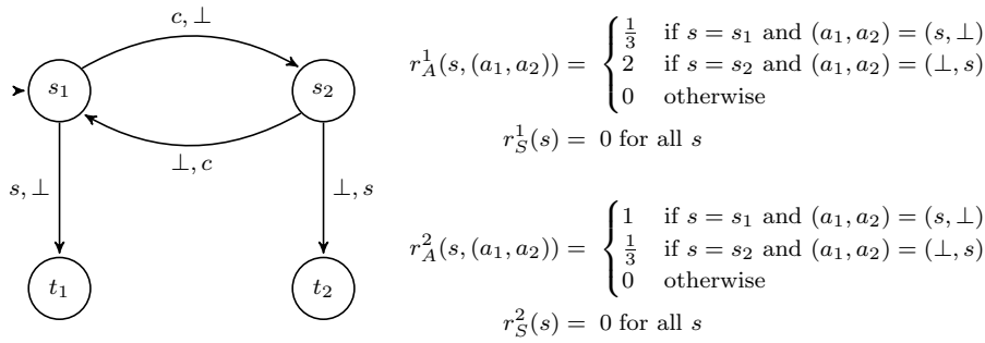
Fig. 15: Counterexample for nonzero-sum expected reachability properties.
