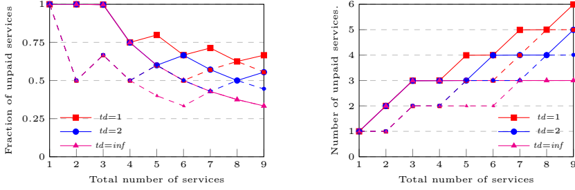
Fig. 11: User-centric network results (CSG/TSG values as solid/dashed lines).
