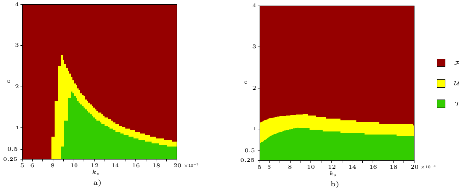
Fig. 10 The computation and results of the threshold synthesis for the DNA walker model, k_s \times c \in [0.005, 0.020] \times [0.25, 4] and different formulas, using volume tolerance \varepsilon = 10\% . a) P_{\geq 0.4}[F^{[30,30]} \text{ finish-correct}] \wedge P_{\leq 0.08}[F^{[30,30]} \text{ finish-incorrect}] , runtime 282.5 s, 3489 subspaces*. b) P_{\geq 0.8}[F^{[200,200]} \text{ finish-correct}] \wedge P_{\leq 0.16}[F^{[200,200]} \text{ finish-incorrect}] , runtime 8.2 h, 47229 subspaces*. Results are obtained by solving the synthesis problem for each sub-formula and by combining the output regions as in Eqn 6. *: derived as the sum of runtimes and subspaces for each sub-formula.
