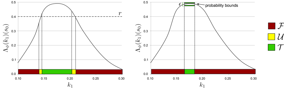
Fig. 2 Synthesis for the birth-death process of Fig. 1. Left: threshold synthesis for P_{\geq 0.4}[\phi] and with volume tolerance \varepsilon = 5\% . Right: max-synthesis with probability tolerance \varepsilon = 2\% .
