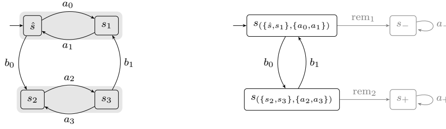
Figure 3 Example of an MDP (left) and its collapsed version (right) with T = \{s_2\} and EC = \{(\{\hat{s}, s_1\}, \{a_0, a_1\}), (\{s_2, s_3\}, \{a_2, a_3\})\} .
