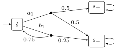
Figure 1 Example MDP where following the upper bounds is wrong.
