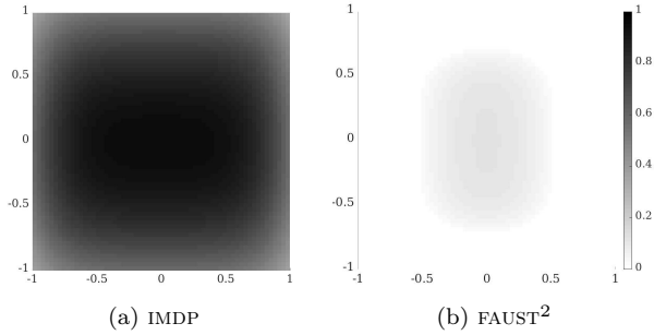
Figure 3: Lower bound probabilities of satisfying \varphi_1 with |Q| = 3721 and k = 2 .
